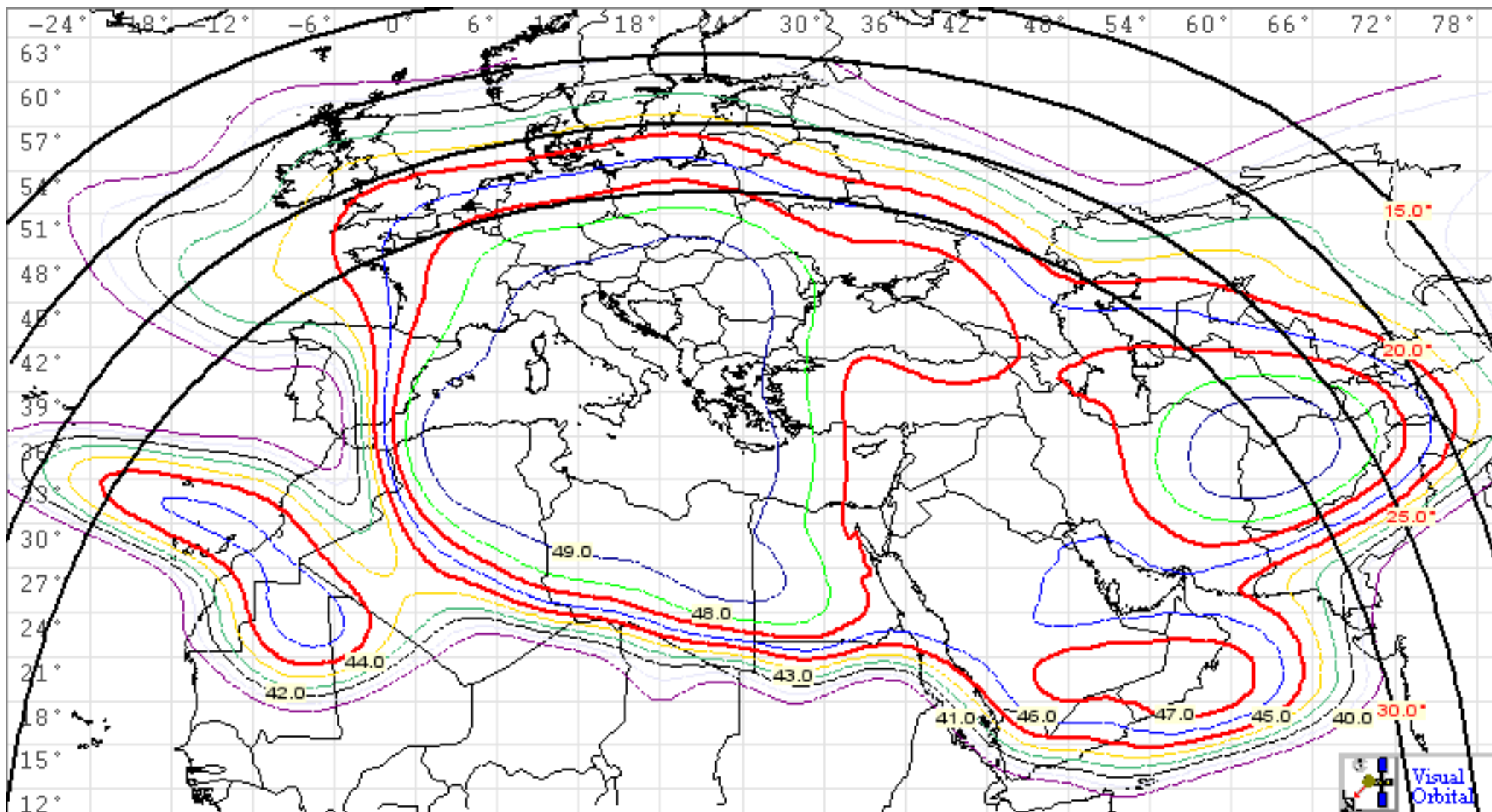
Figure 2: Satellite EIRP (dBW) for Transponder F2 of W6 Satellite at 21.5° East
