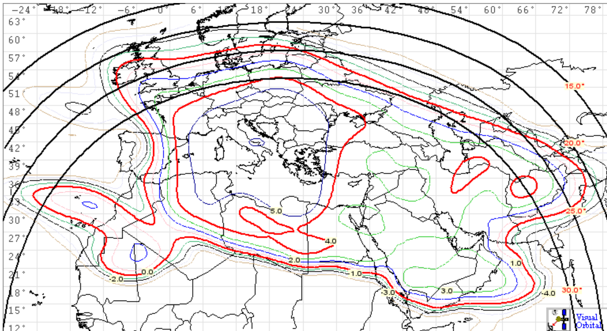
Figure 1: Satellite G/T (dB/K) for Transponder F2 of W6 Satellite at 21.5° East
